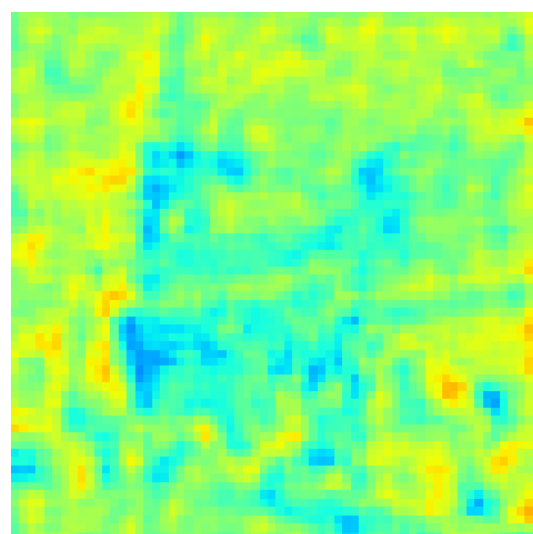
Similarity Map
