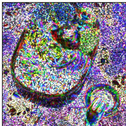
StableGuard
