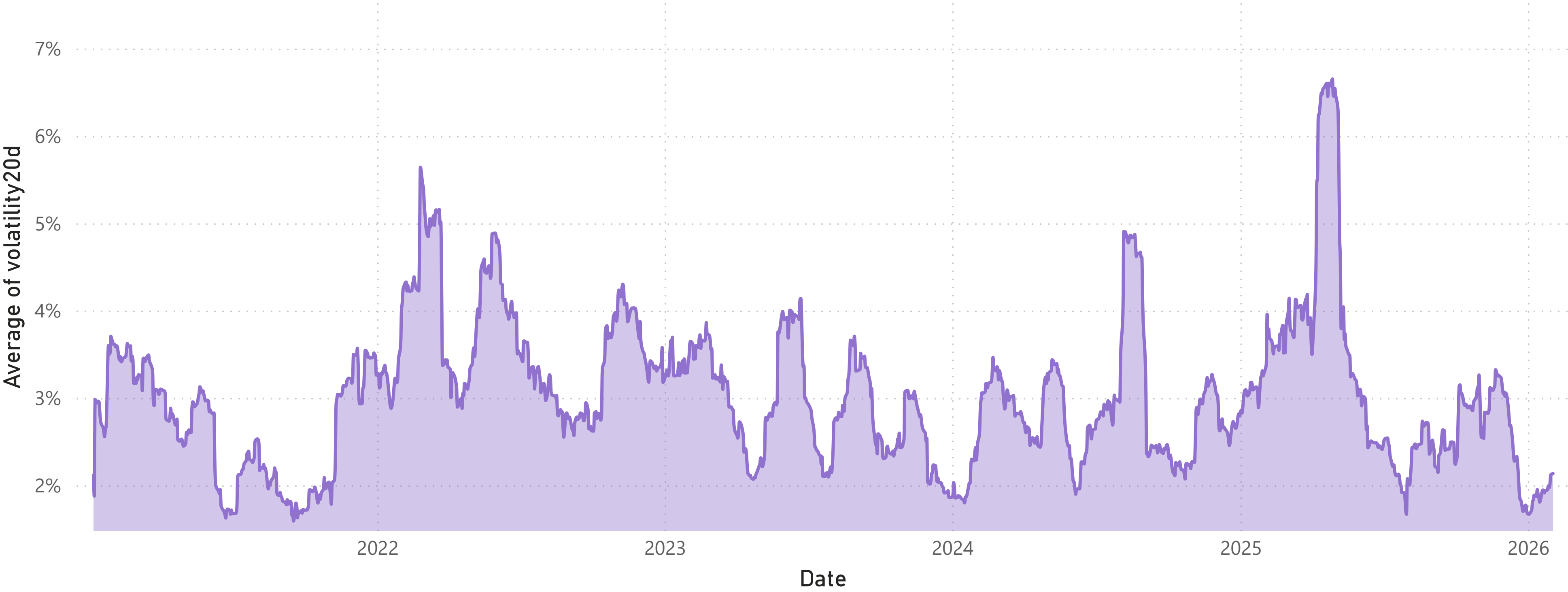
Average 20-Day Volatility Over Time
