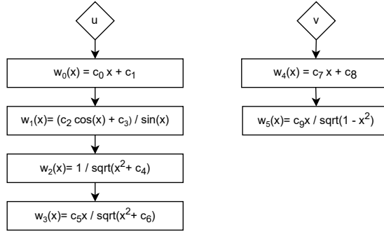
Fig. 1. The warp pipeline of spherical rectangle sampling [14].
