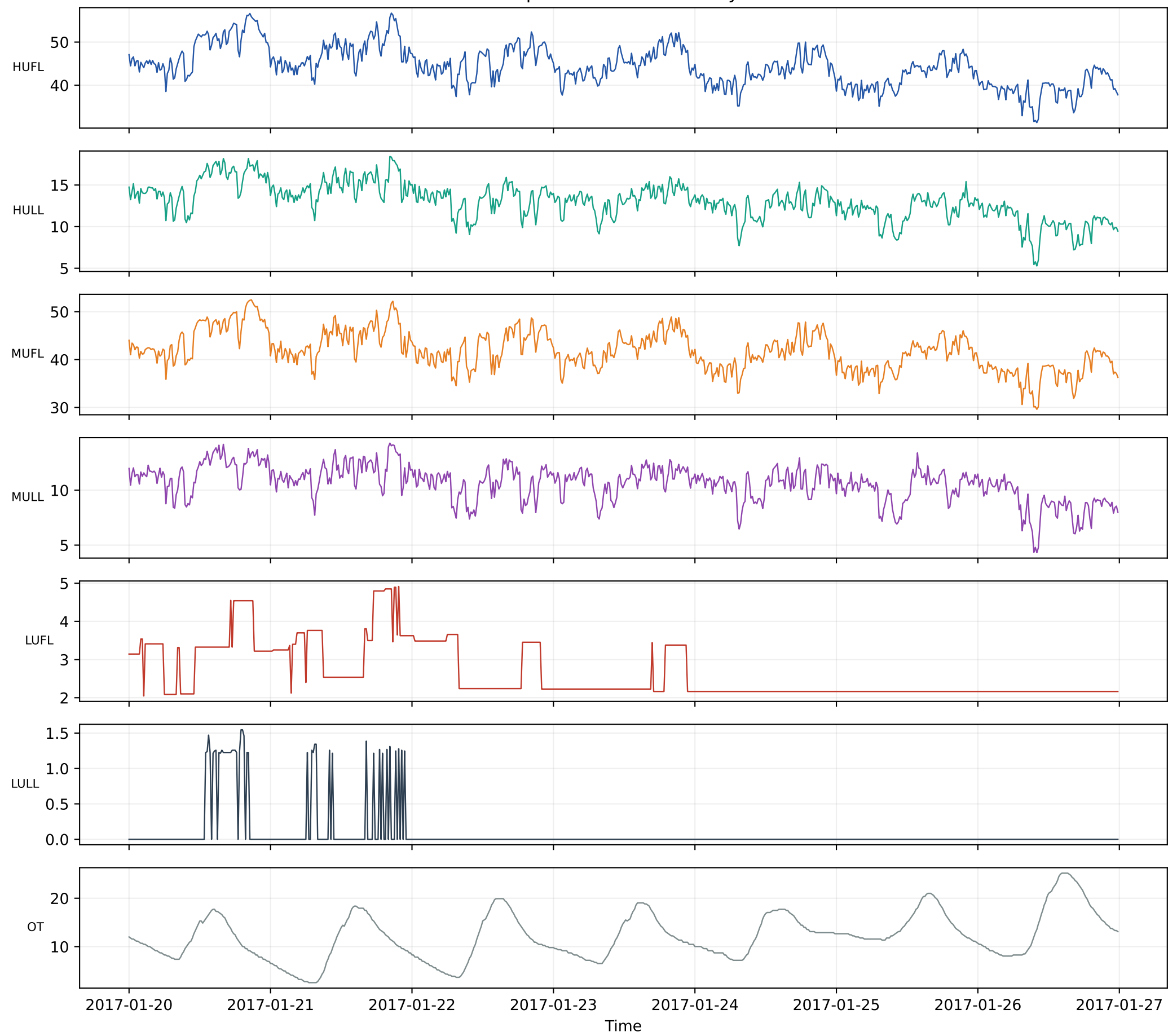
ETTm2: representative seven-day window
