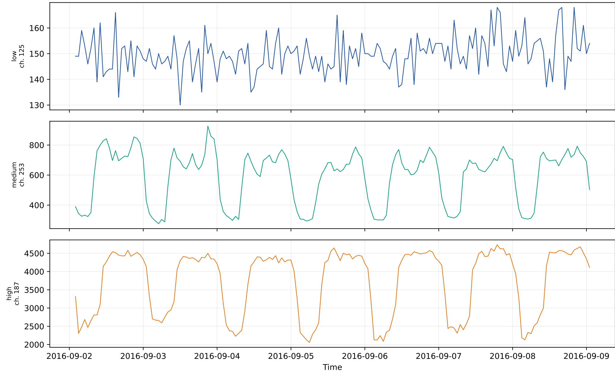
Electricity: representative low-, medium-, and high-activity channels
