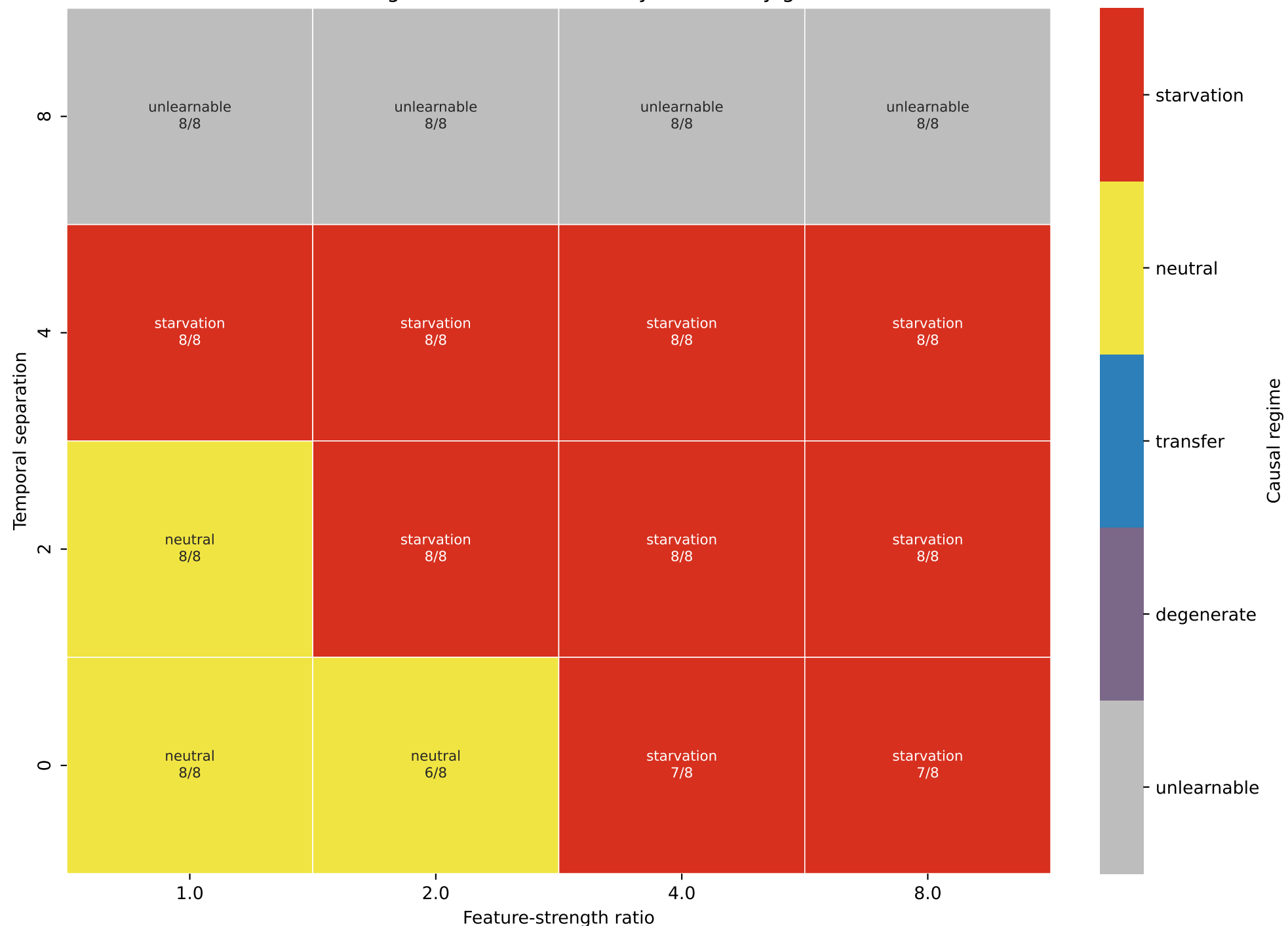
Causal regime after the weak-only learnability gate
