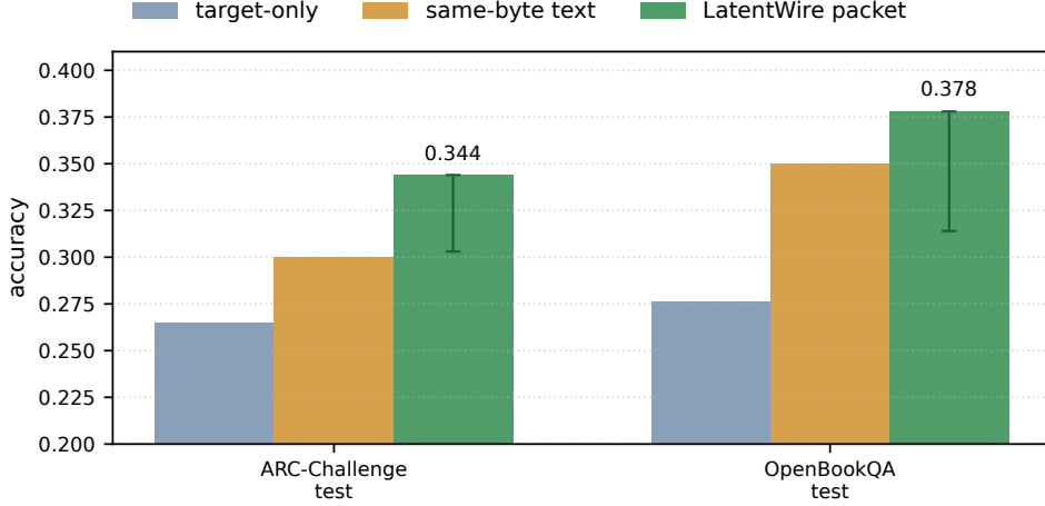
Figure 2: Packet accuracy against target-only and same-budget structured text controls. Error bars show the lower paired-bootstrap lift above target-only; upper uncertainty is omitted for readability because the gate is one-sided.
