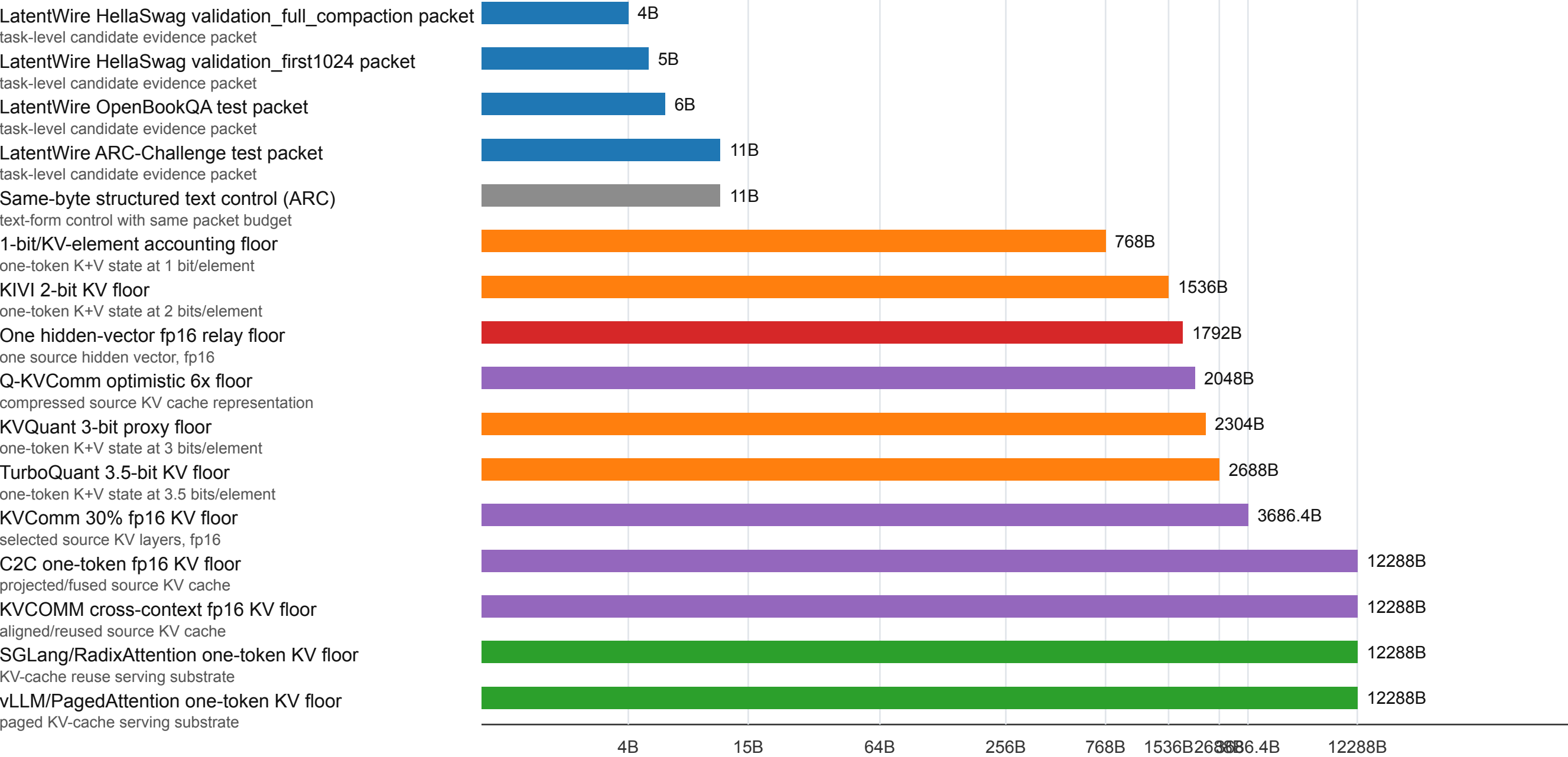
Log-scale framed or state bytes per request; KV rows are byte floors, not native wins
