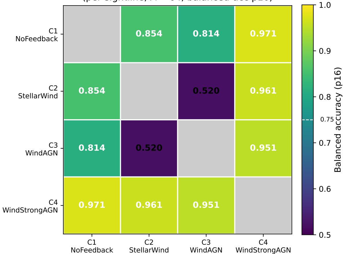
Pairwise distinguishability lattice (per-sightline, M = 64 , balanced-acc p16)
