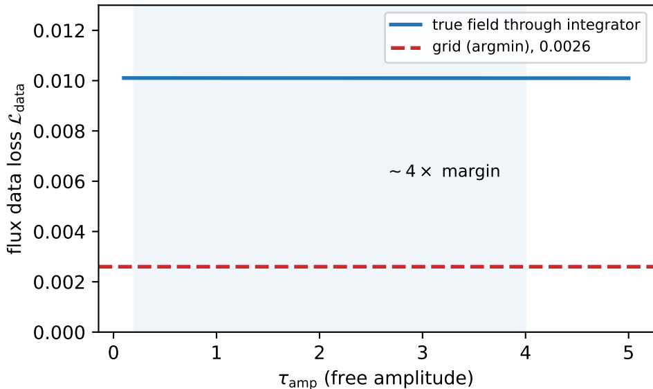
K2: the grid fits flux better than the true field ( z = 0.3 , P_1 , G = 192 , log-space flux loss)
