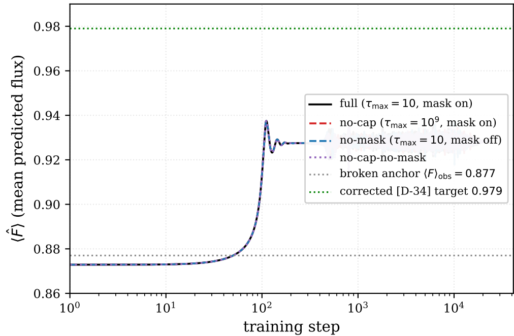
(b) mean predicted flux \langle \hat{F} \rangle vs. step
