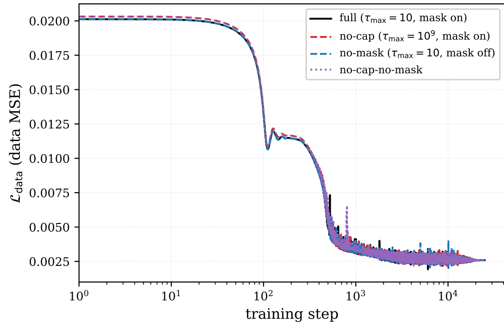
(a) data MSE \mathcal{L}_{\text{data}} vs. step
