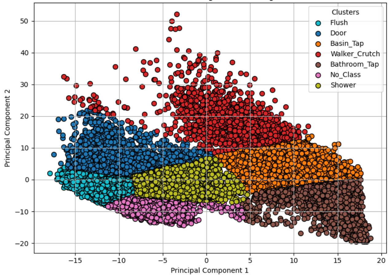
PCA + KMeans Clustering (After Training ACDNet)
