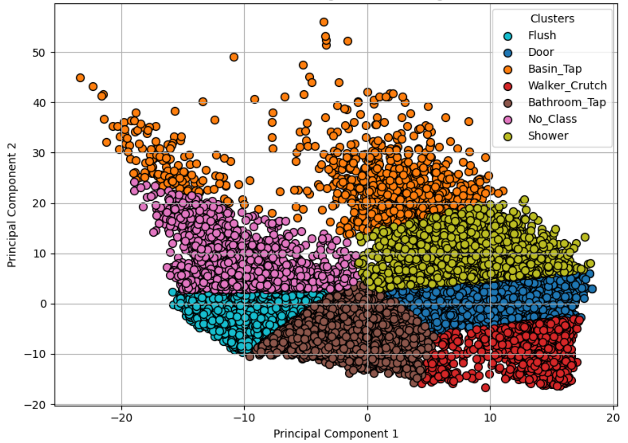
PCA + KMeans Clustering (Before Training ACDNet)
