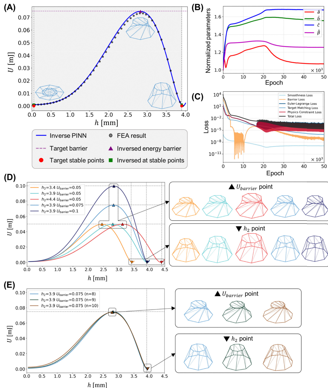
Fig. 7 Bistable energy programming with minimal input. (A) Representative case: h_1 = 0 , h_2 = 3.9 , U_{\text{barrier}} = 0.075 mJ, domains [0, 4] . (B) Evolution of normalized parameters ( a , b , c , \beta ) for case in (A). (C) Loss convergence for case in (A). (D) Five design variations with n = 8 : three cases with h_2 = 3.4 , 3.9 , 4.4 (domains [0, 3.5] , [0, 4] , [0, 4.5] ; U_{\text{barrier}} = 0.05 mJ) and two cases with U_{\text{barrier}} = 0.075 , 0.1 mJ (domain [0, 4] ; h_2 = 3.9 ). Right panels show 3D structures at barrier and second stable states. (E) Polygon number variation ( n = 8, 9, 10 ) for identical targets: h_1 = 0 , h_2 = 3.9 , U_{\text{barrier}} = 0.075 mJ, domain [0, 4] . Right panels show corresponding 3D structures.
