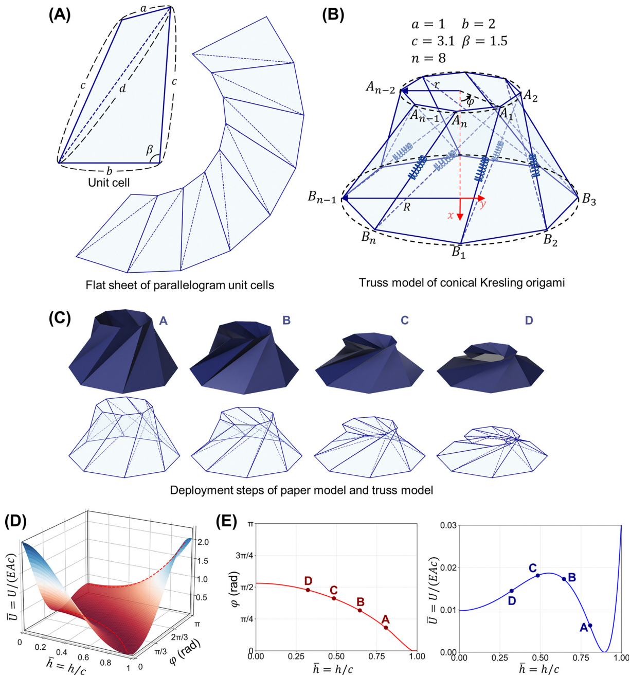
Fig. 1 Geometric modeling and energy landscape of conical Kresling origami (CKO). (A) Unit cell and flat crease pattern with geometric parameters: a , b , c , d , and \beta . (B) 3D CKO structure and truss model showing vertices ( A_i, B_i ), radii ( r , R ), and rotation angle \phi ( a = 1 , b = 2 , c = 3.1 , \beta = 1.5 , n = 8 ). (C) Compression sequence (A)–(D) with paper model (top) and truss model (bottom). (D) Energy landscape U(\bar{h}, \phi) with torque-free equilibrium paths (red dashed lines). (E) Energy U and rotation angle \phi versus normalized height \bar{h} , with points A–D corresponding to stages in (C).
