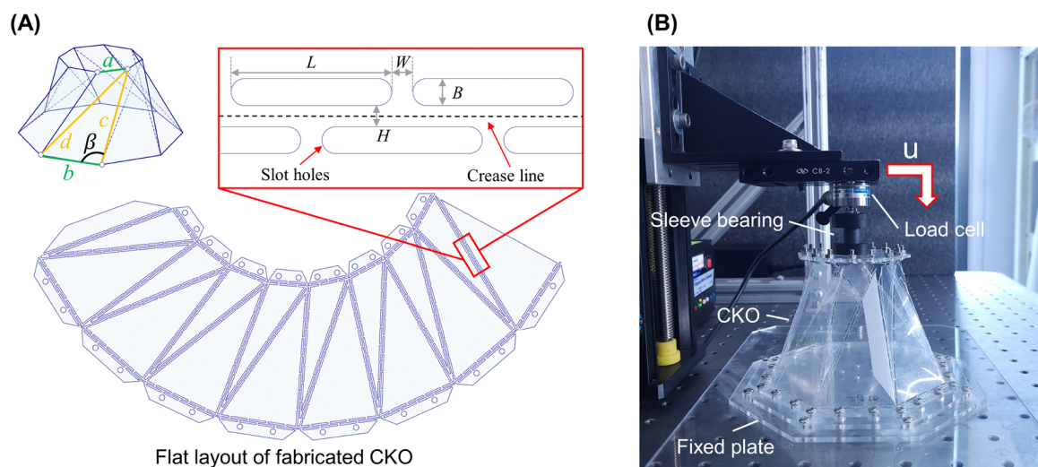
Fig. 3 Geometry and experimental setup of a CKO. (A) Geometric design and crease parameters of the CKO unit. (B) Experimental setup for uniaxial compression test of the CKO.
