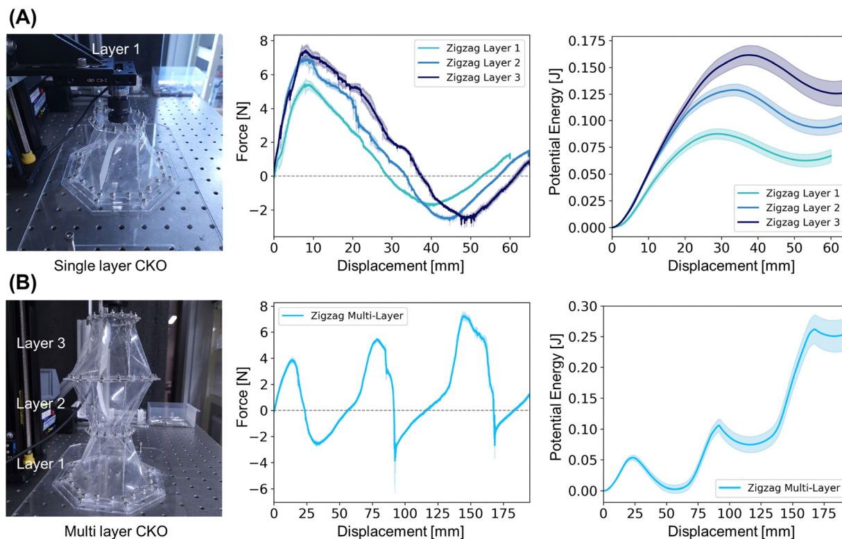
Fig. 9 Experimental validation of zigzag configuration. (A) Individual layer tests: layer 1 specimen photograph at initial state with force-displacement and energy-displacement curves for all three layers. (B) Three-layer assembly test: initial state photograph with force and energy response during compression showing three distinct peaks and energy accumulation.
