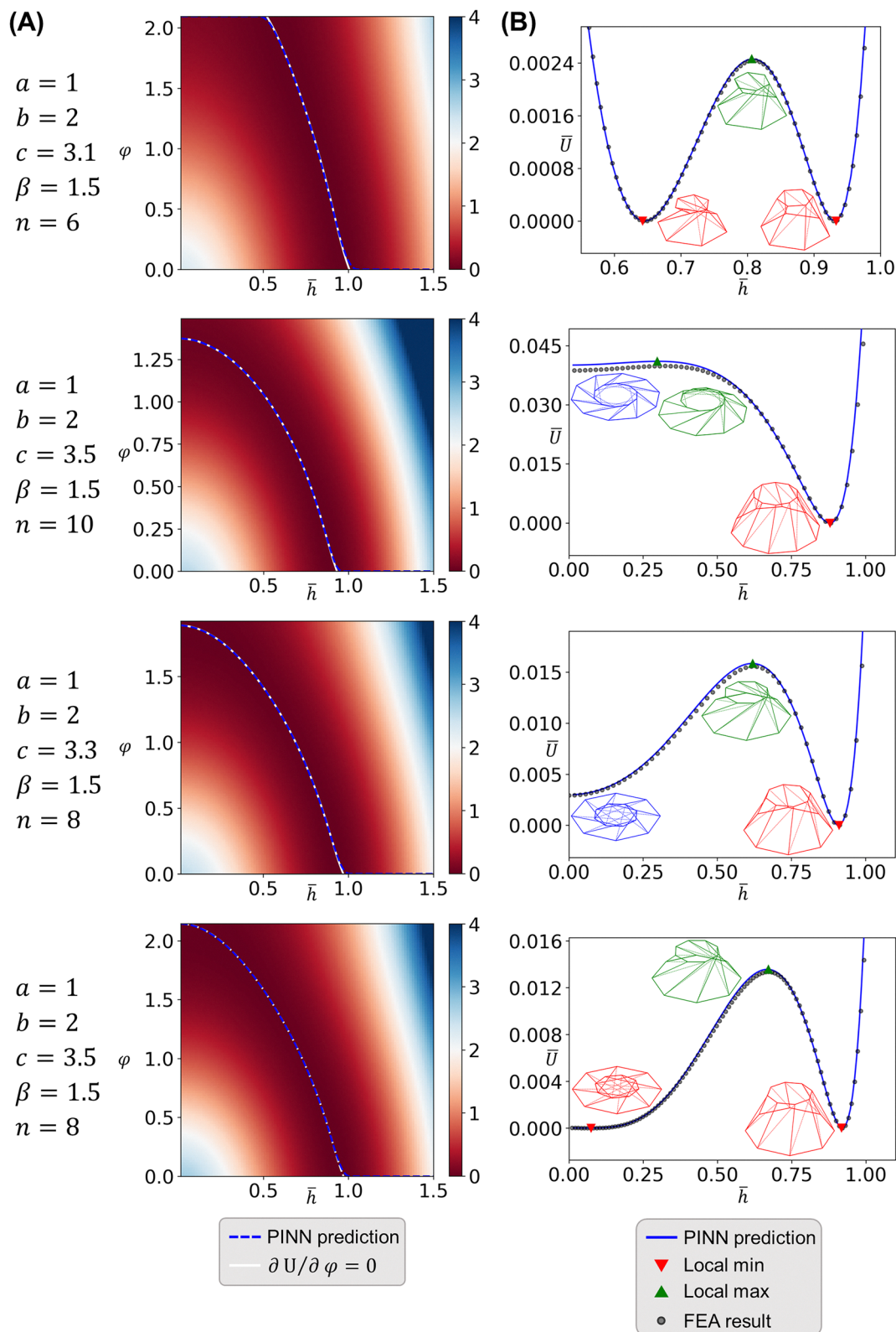
Fig. 4 Forward prediction of energy landscapes for diverse CKO geometries. (A) Energy fields \bar{U}(\bar{h}, \varphi) for four representative cases with torque-free equilibrium paths (white solid lines: \partial U / \partial \varphi = 0 ) and PINN predictions (blue dashed lines). (B) Energy curves \bar{U}(\bar{h}) showing PINN predictions (blue solid lines) versus FEA results (black dots). Red triangles mark stable minima and green triangles indicate energy barriers, with corresponding 3D CKO structures embedded at these critical points. From top to bottom: Case 1 exhibits bistability with two zero-energy states; Case 2 shows monostability; Case 3 demonstrates asymmetric bistability with non-zero energy minimum (blue structure); Case 4 shows bistability with zero-energy states, one at \bar{h} = 0 (fully folded).
