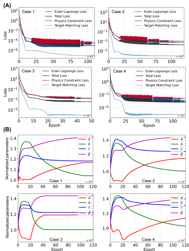
Fig. 6 Convergence behavior during inverse design training. (A) Evolution of loss components over training epochs for the four representative cases from Fig. 5. (B) Normalized structural parameters ( \hat{a}, \hat{b}, \hat{c}, \hat{\beta} ) plotted against training epochs, showing stable convergence trends.
