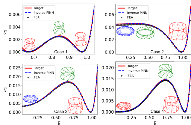
Fig. 5 Inverse design based on target energy curves. Comparison of normalized energy curves \hat{U}(\hat{h}) for four representative cases, showing target profiles (red solid lines), inverse-designed PINN predictions (blue dashed lines), and FEA validation results (black dots).
