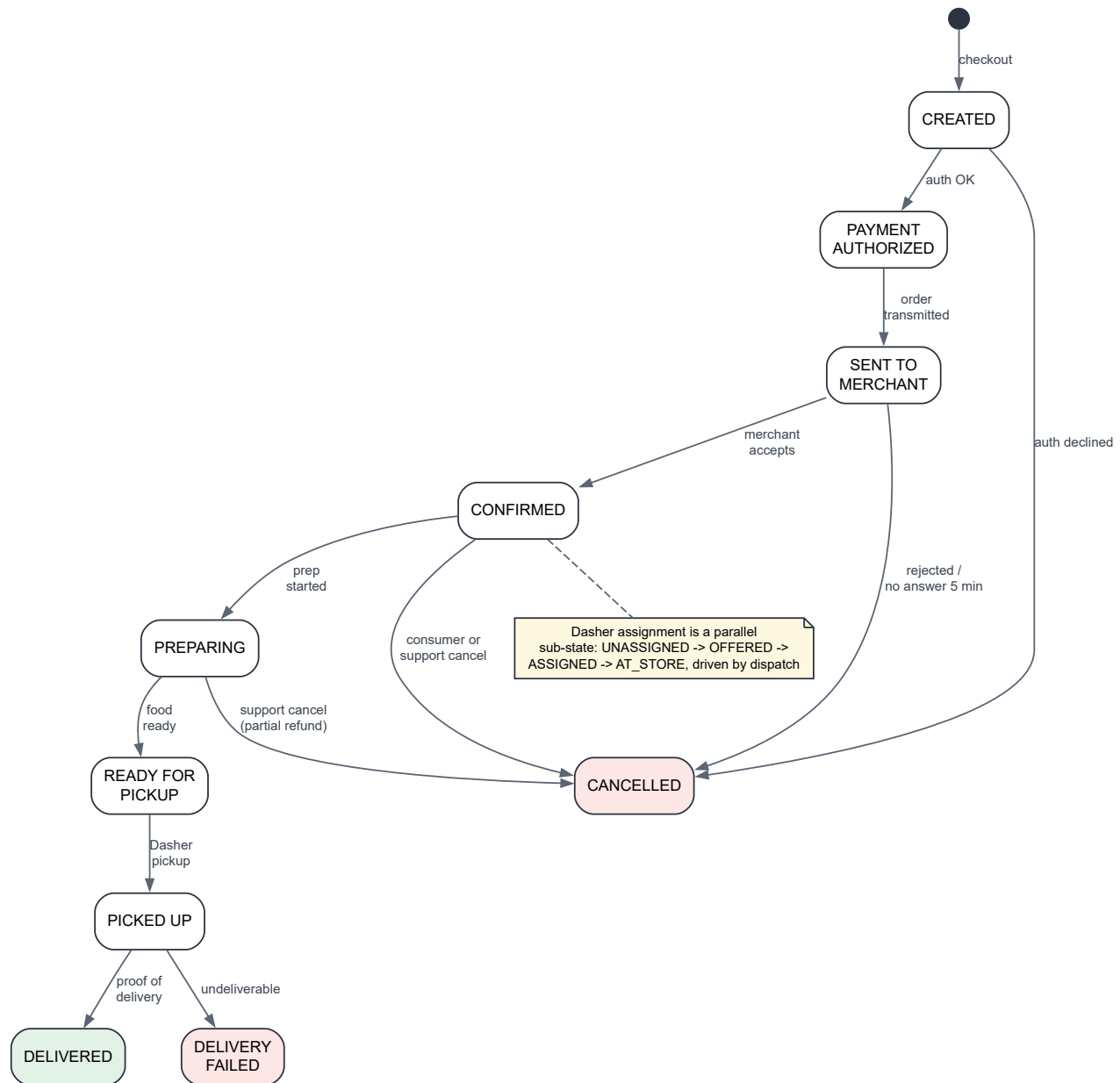
Figure 3. Order lifecycle state machine (FR-05)
