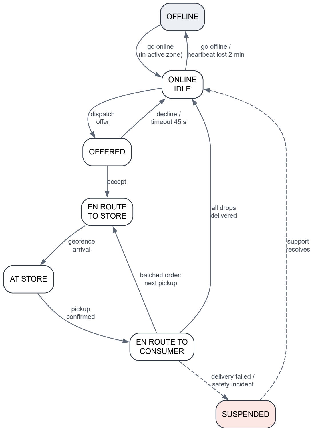
Figure 4. Dasher state machine (FR-08)
