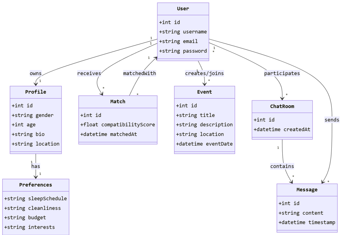
Figure 2.4: Class Diagram
