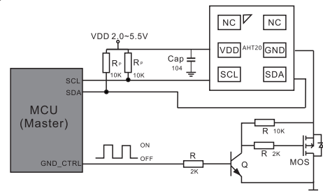
Figure 15-2 Typical application circuit ②, AHT20 operation is controlled by whether GND is grounded.
