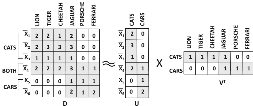
(a) Two-way factorization
