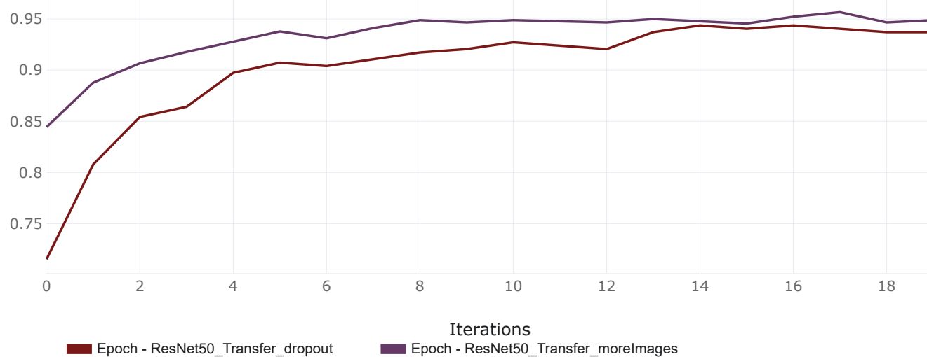
Validation Chart
