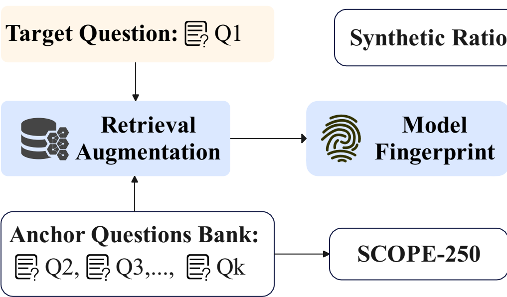
(a) Fingerprint Construction
