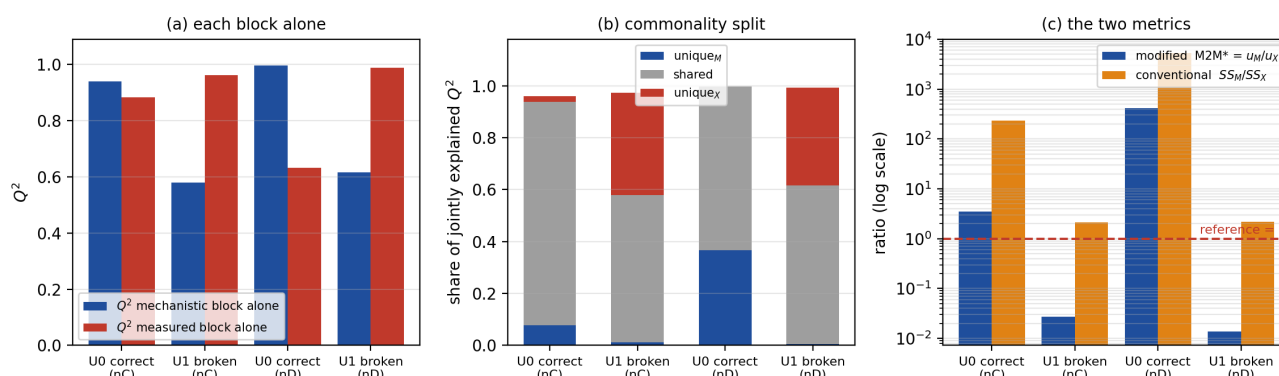
Figure 7 — (a) what each block predicts on its own; (b) the commonality split; (c) both metrics on a log scale against the intrinsic reference at 1. The modified metric puts the correct and the broken model on opposite sides of that line; the conventional one does not.
