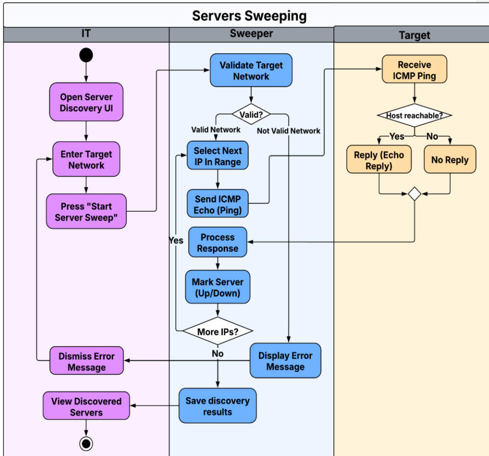
Figure 37: Activity diagram for the server sweeping process.
