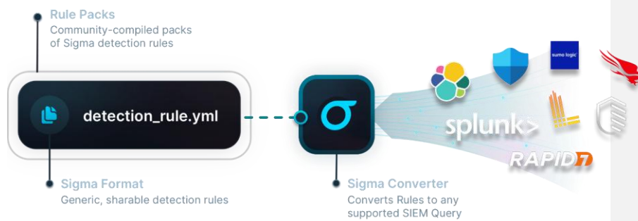
Figure 8: Sigma rules where generic YAML-based detection rules are bundled into rule packs and passed through a SIEM-specific queries for platforms such as Splunk, Elastic, and other security tools.
