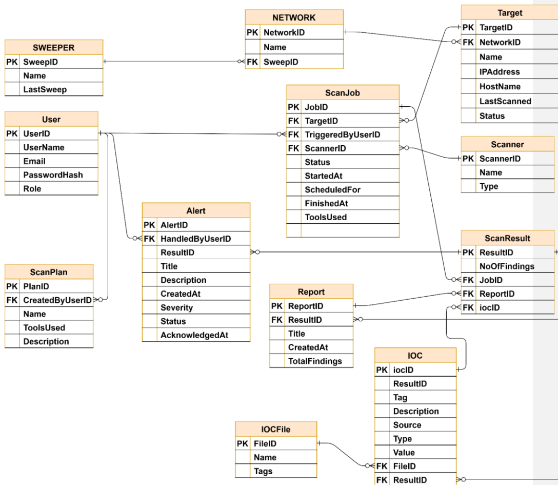
Figure 44: Relational ER Diagram (Logical Data Model) showing the main tables with their attributes, primary keys and foreign-key relationships.
