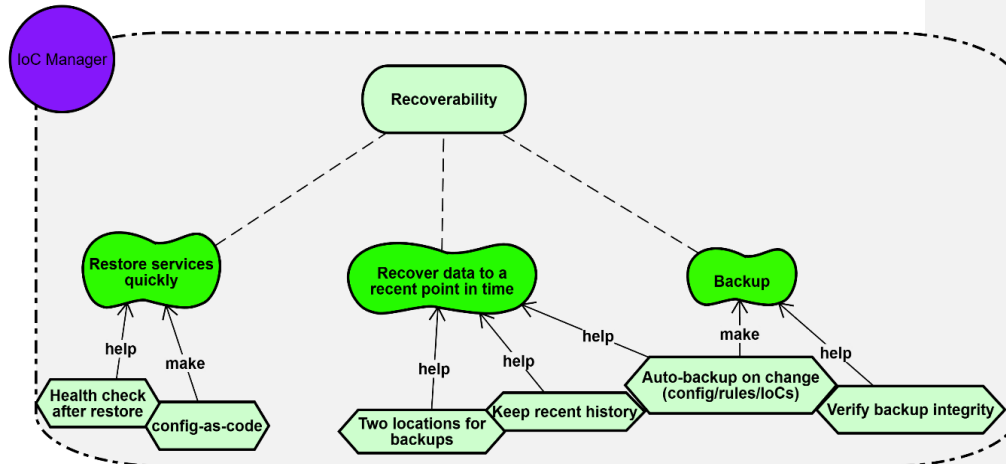
Figure 19: “Recoverability” reliability model, linking the high-level goal of “Recoverability” to its qualities and the concrete tasks and mechanisms that make or help achieve each quality.
