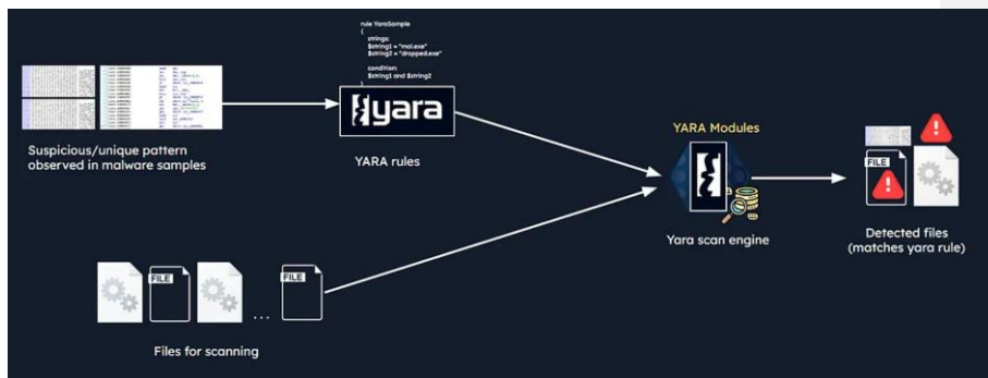
Figure 7: YARA rule-based detection workflow. (Bavarva, n.d.).
