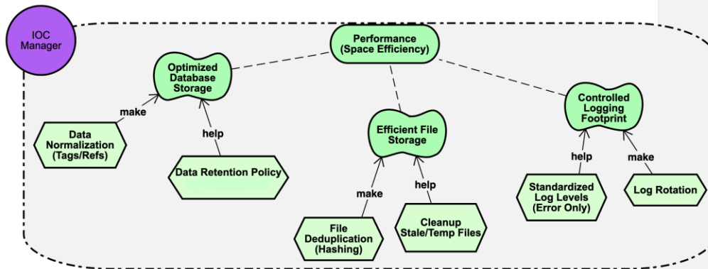
Figure 26: “Performance-space” model, linking the high-level goal of “Performance-space” to its qualities and the concrete tasks and mechanisms that make or help achieve each quality.
