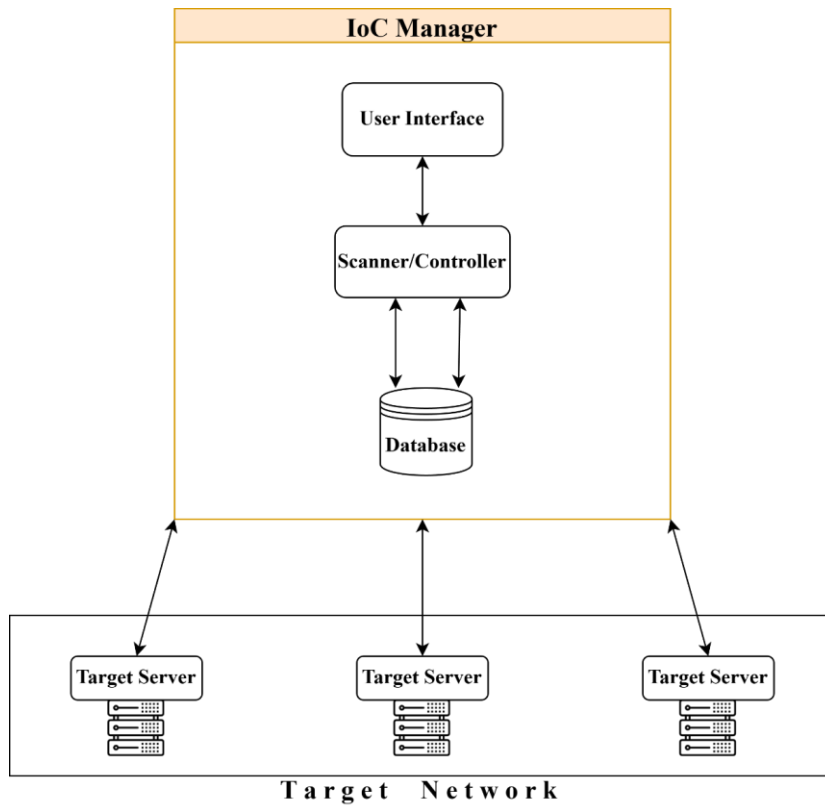
Figure 32: High-level architectural design of our IoC Manager.
