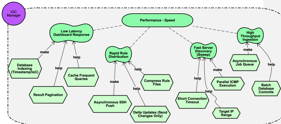
Figure 25: “Performance-speed” model, linking the high-level goal of “Performance-speed” to its qualities and the concrete tasks and mechanisms that make or help achieve each quality.
