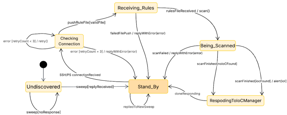
Figure 36: State machine diagram for the target server, showing how the target transitions between the different states.
