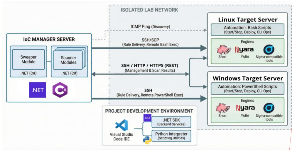
Figure 31: Visual overview of the IoC Manager environment and project constraints.
