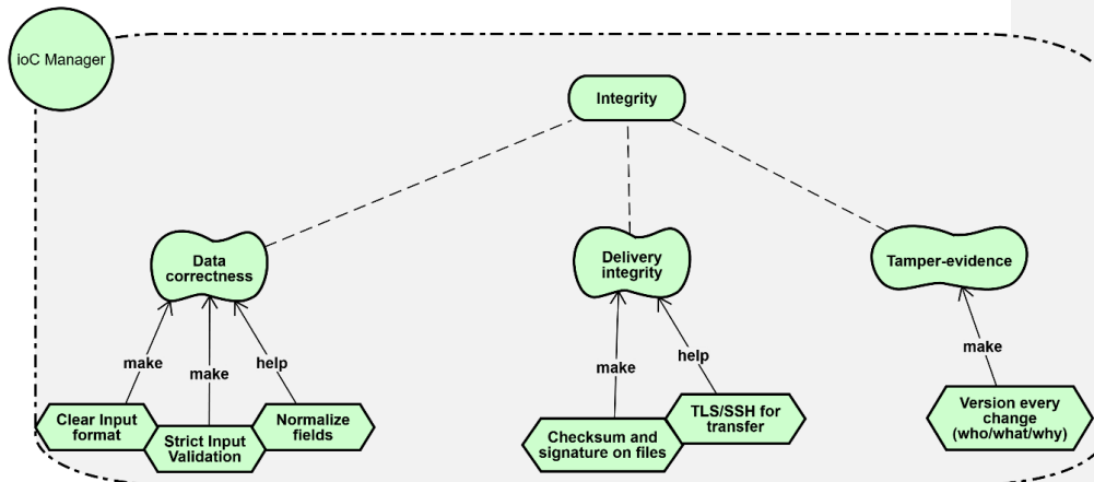
Figure 23: “Integrity” security model, linking the high-level goal of “Integrity” to its qualities and the concrete tasks and mechanisms that make or help achieve each quality.
