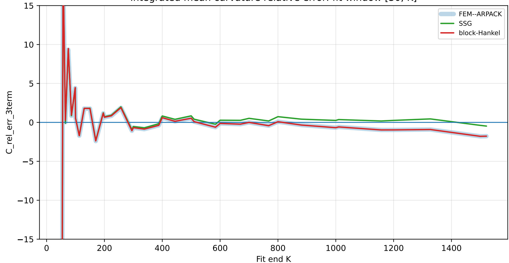
Integrated mean curvature relative error: fit window [30, K]
