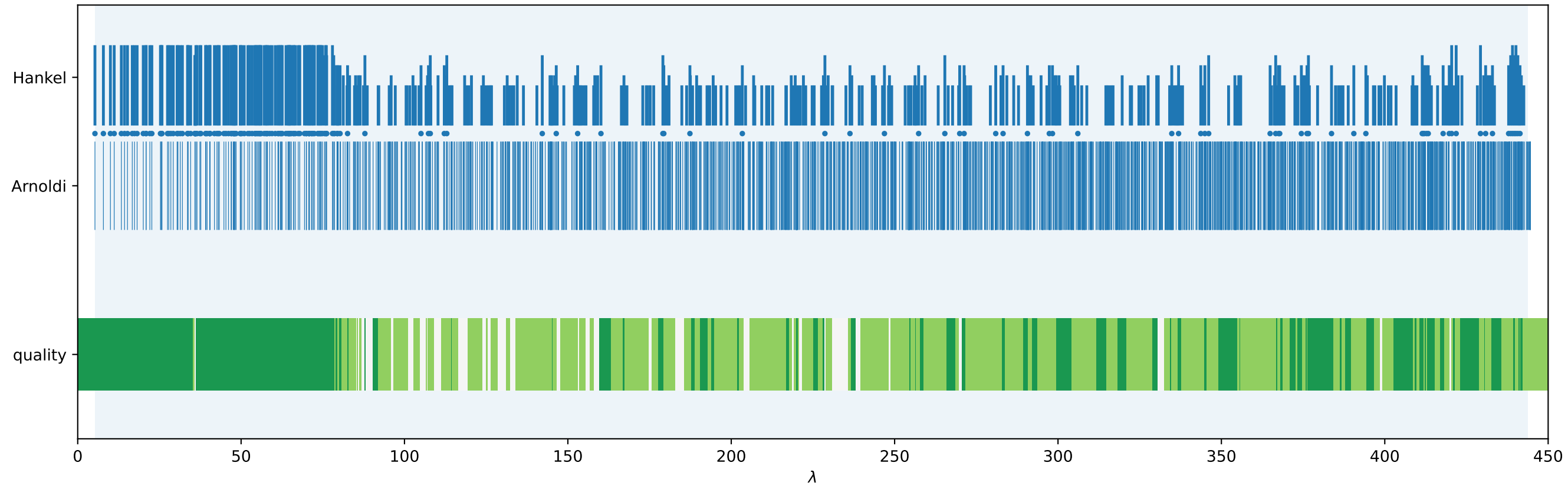
Stable Hankel landmarks and Arnoldi reference spectrum
