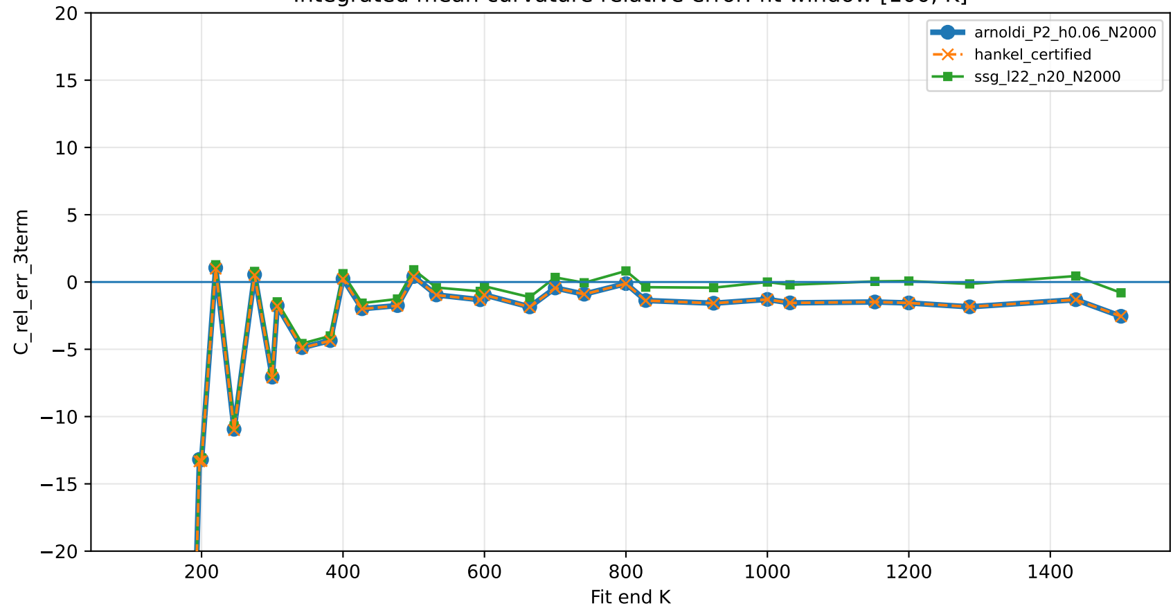
Integrated mean curvature relative error: fit window [100, K]
