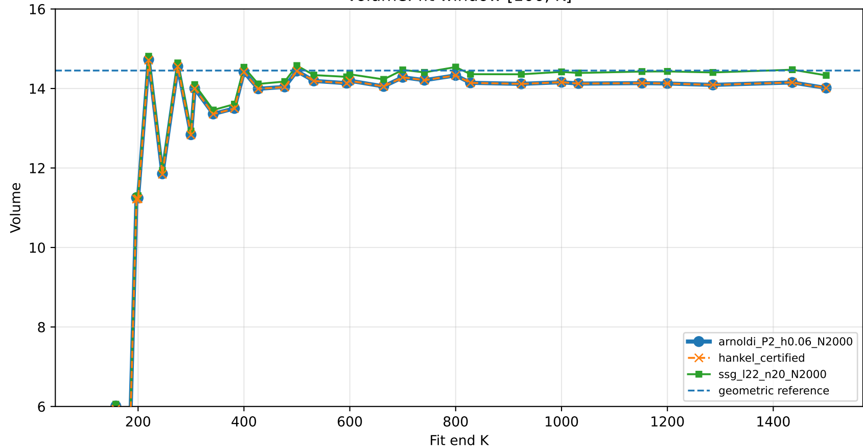
Volume: fit window [100, K]
