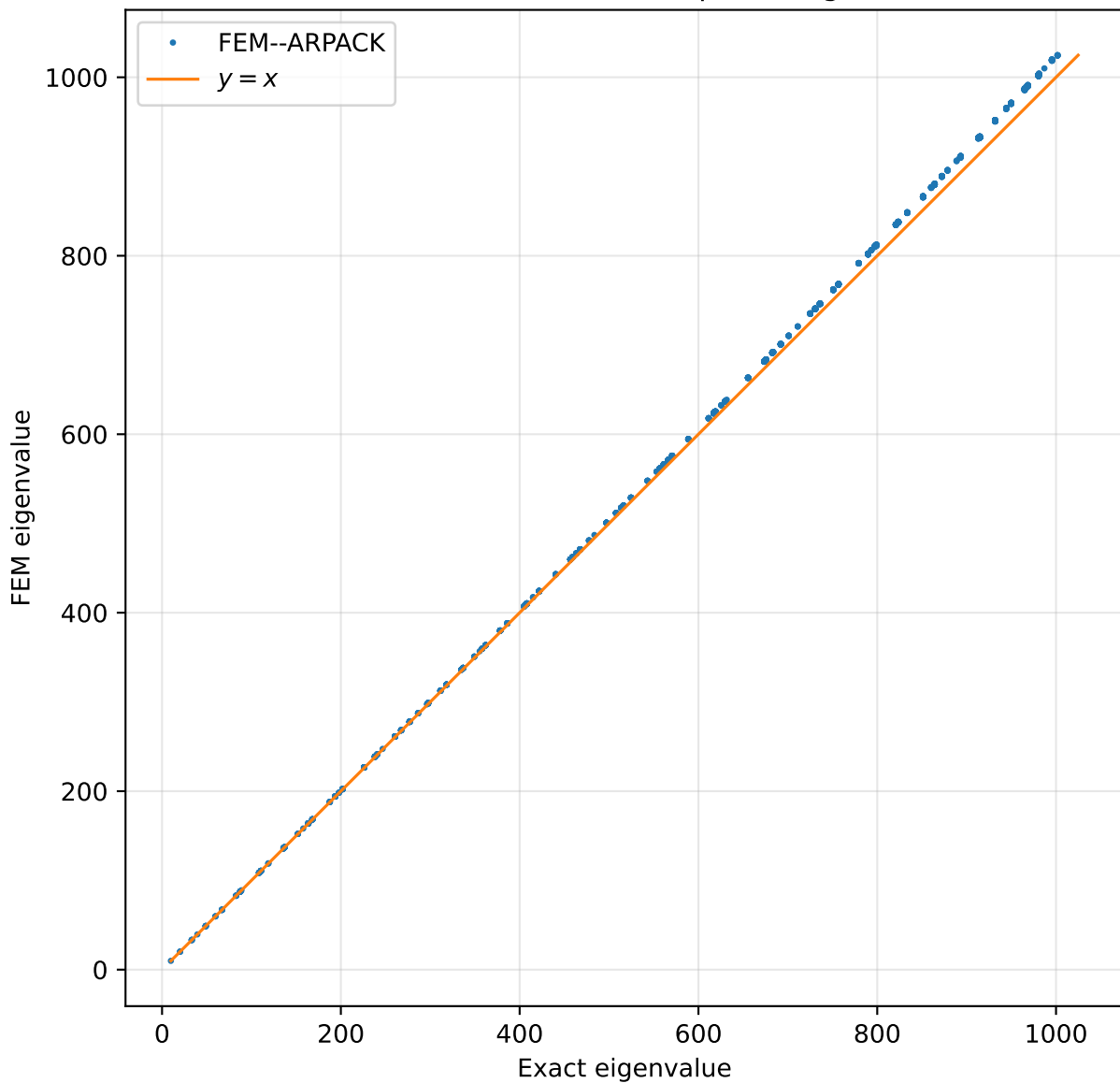
Unit ball: exact vs. FEM-computed eigenvalues
