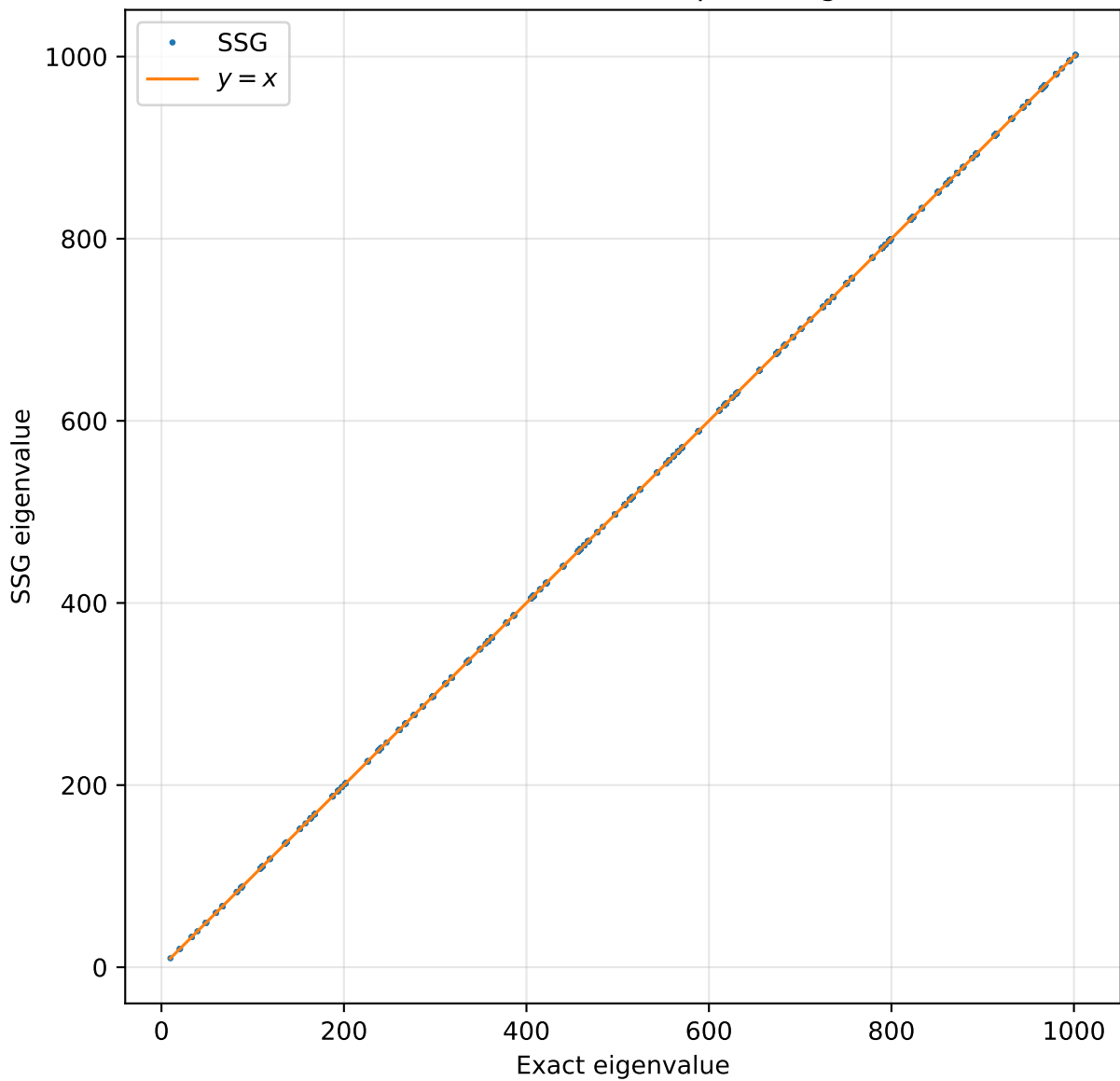
Unit ball: exact vs. SSG-computed eigenvalues
