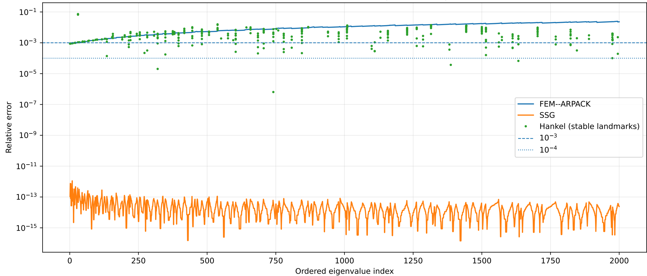
Unit ball: FEM--ARPACK, SSG, and Hankel against exact ground truth
