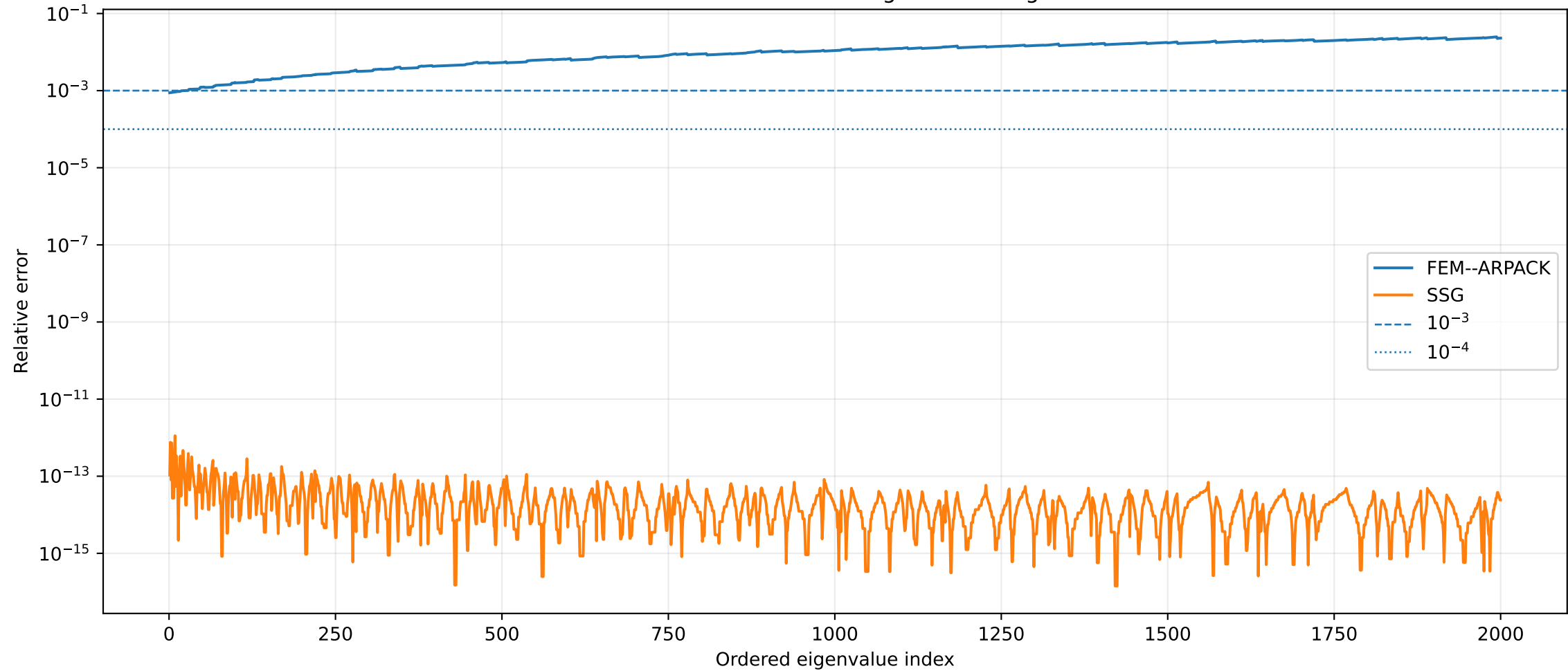
Unit ball: FEM--ARPACK and SSG against exact ground truth
