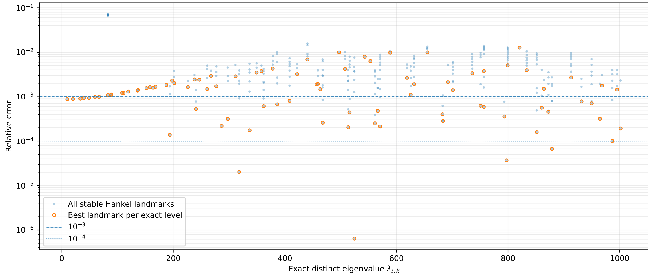
Unit ball: stable Hankel landmarks against exact distinct levels
