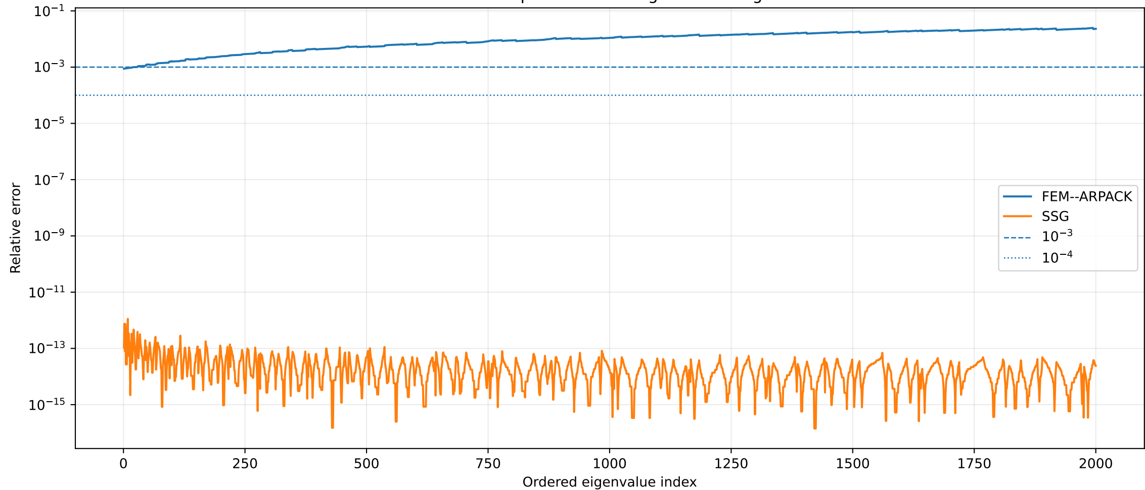
Unit ball: ordered-spectrum error against exact ground truth
