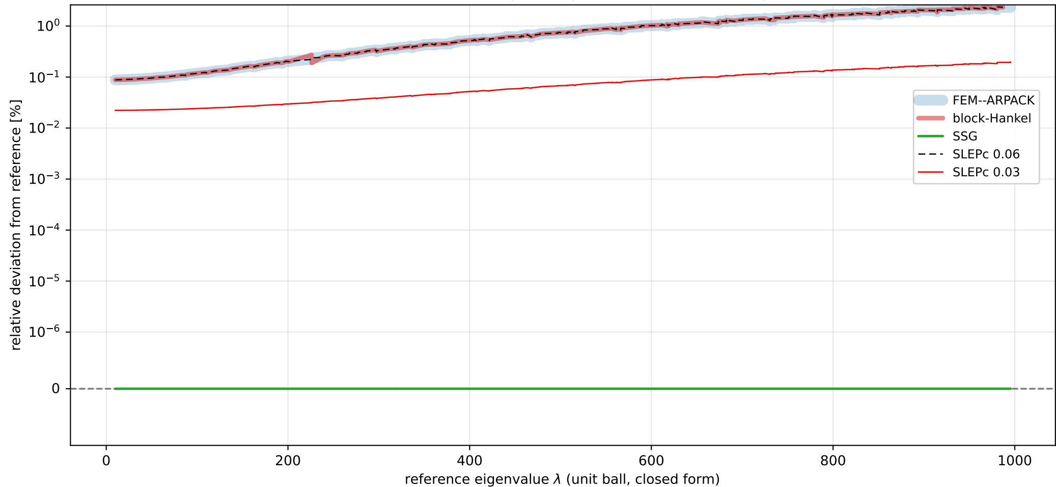
Unit ball: deviation of computed spectra from the exact spectrum
