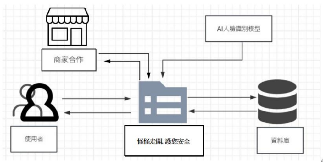
Figure 1: System Architecture
