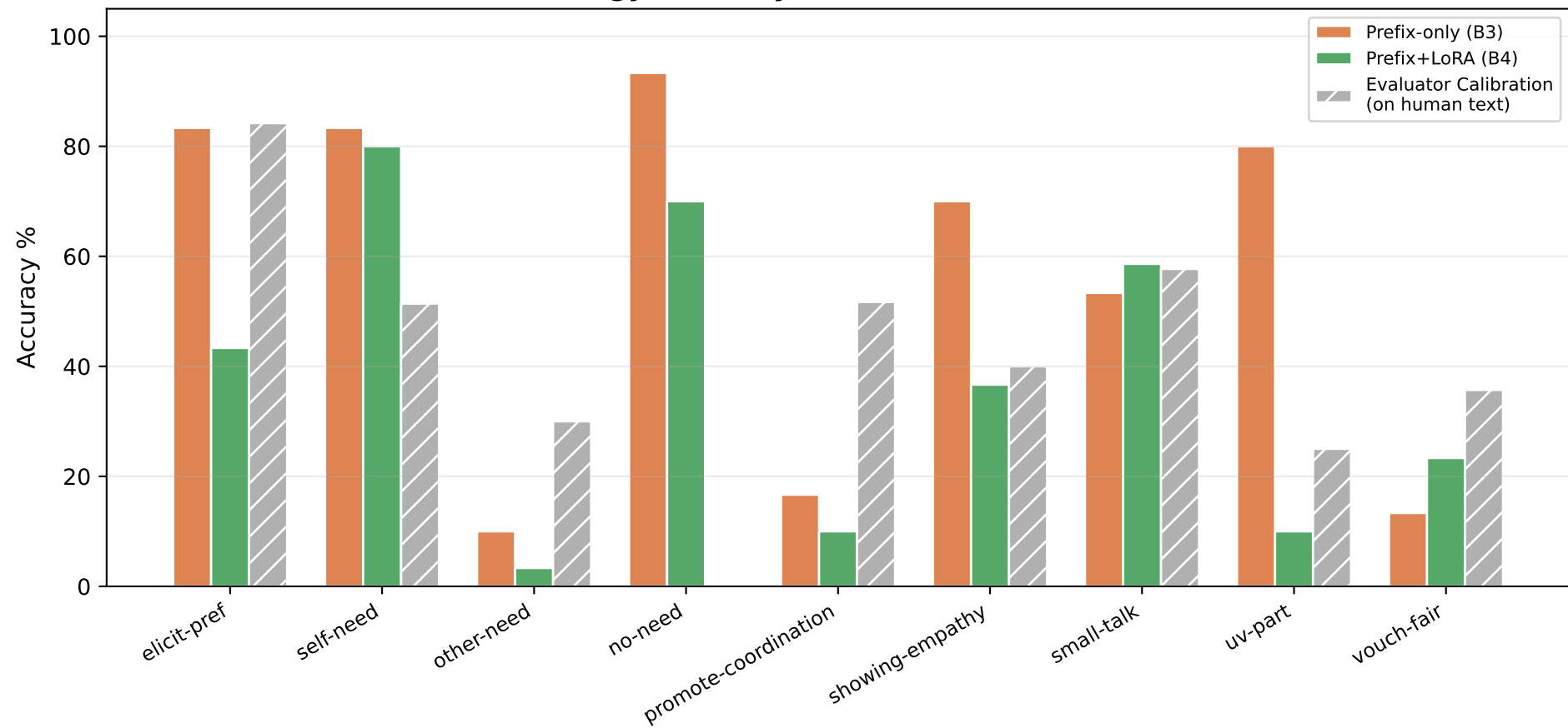
Per-Class Strategy Accuracy: B3 vs B4 vs Evaluator Calibration
