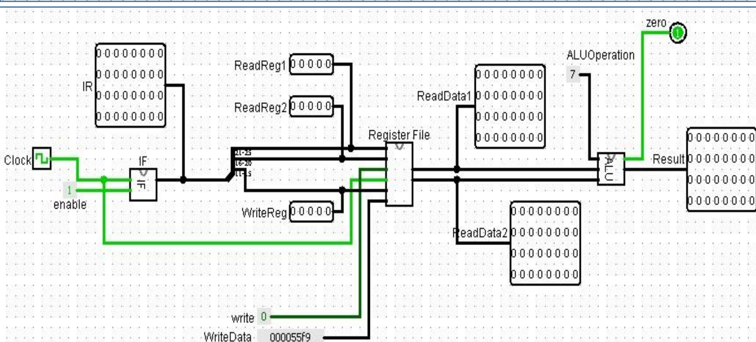
Instruction Fetch, Register File and ALU sub-circuits
