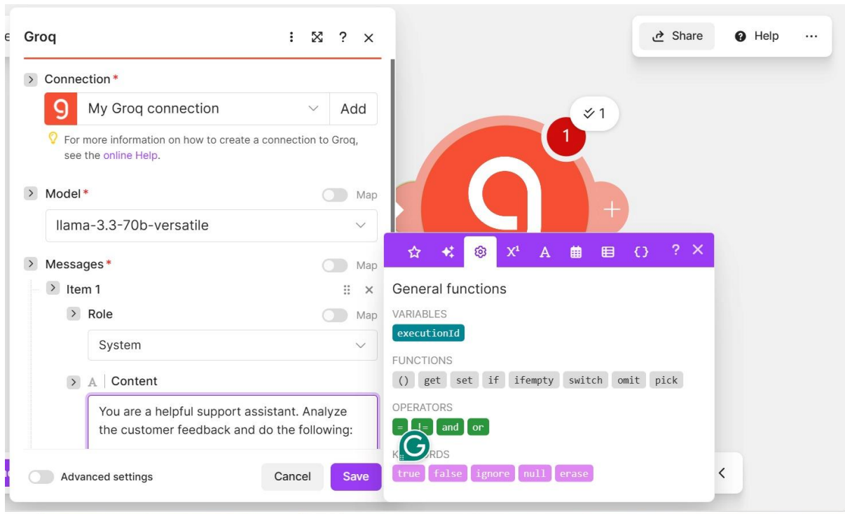
Fig. 3 Groq module: System role message defining the AI's persona and instructions.
