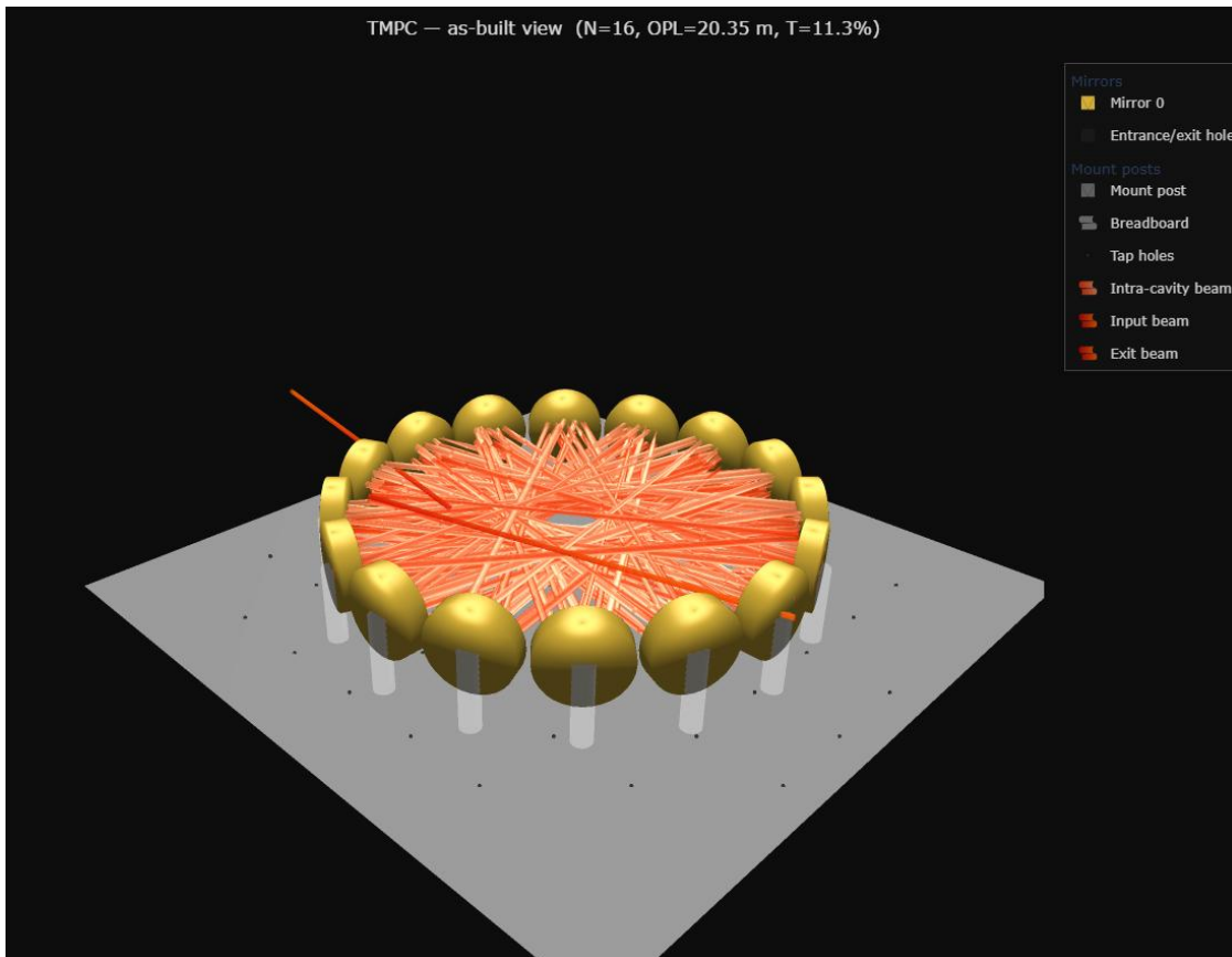
Fig. 4. As-built rendering of the headline design: sixteen 25.4 mm mirrors in a one-piece machined ring; laser collimator, mode-matching lens and detector all mount behind M0, the exit beam leaving 22.5° from the injection axis.
