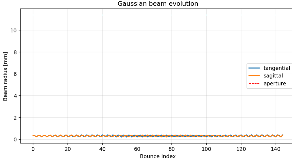
Fig. 3. Tangential and sagittal 1/e^2 beam radii at each bounce under mode-matched injection: the beam rides the cell eigenmode at 0.21–0.42 mm for all 144 chords, an order of magnitude below the 11.4 mm clear aperture.
