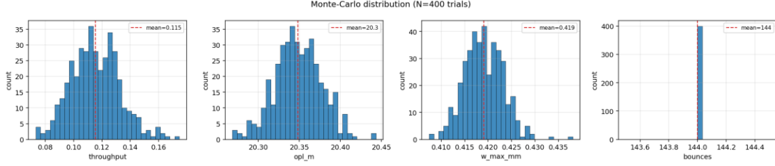
Fig. 7. Monte-Carlo distributions for the headline design at research-grade tolerances (400 trials): traversal count is invariant at 144; OPL and exit drift remain within operational bounds in every trial.
