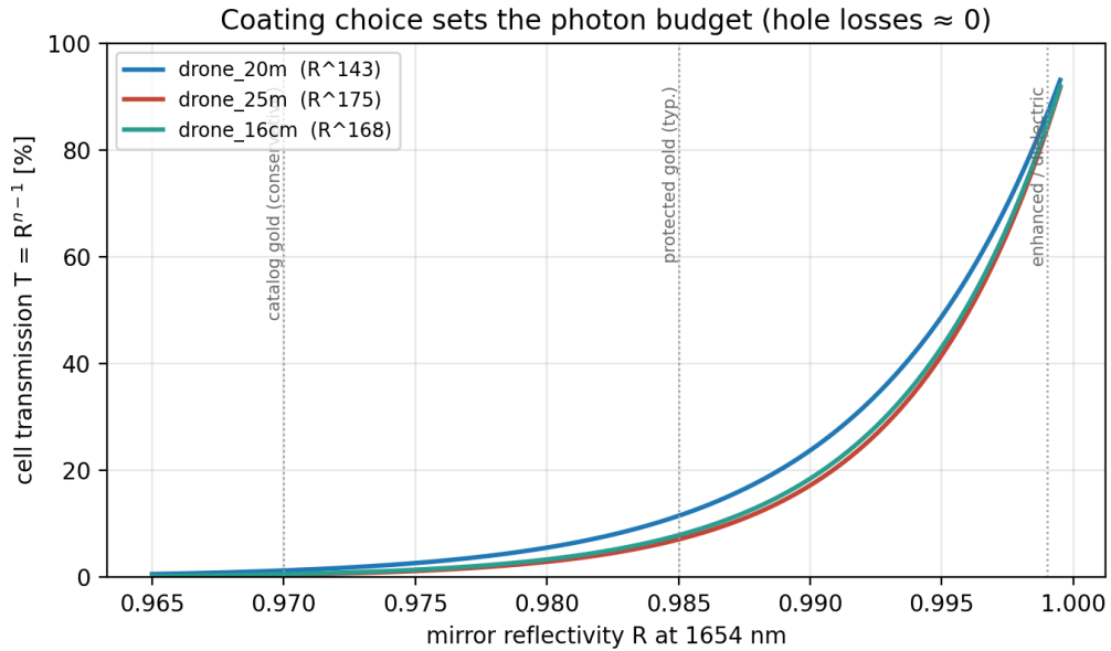
Fig. 6. Coating choice sets the photon budget: with the coupling hole rendered lossless by mode matching, transmission is exactly R to the power (chords - 1 ) for every design. Vertical guides mark conservative catalogue gold, typical protected gold, and enhanced/dielectric coatings.
