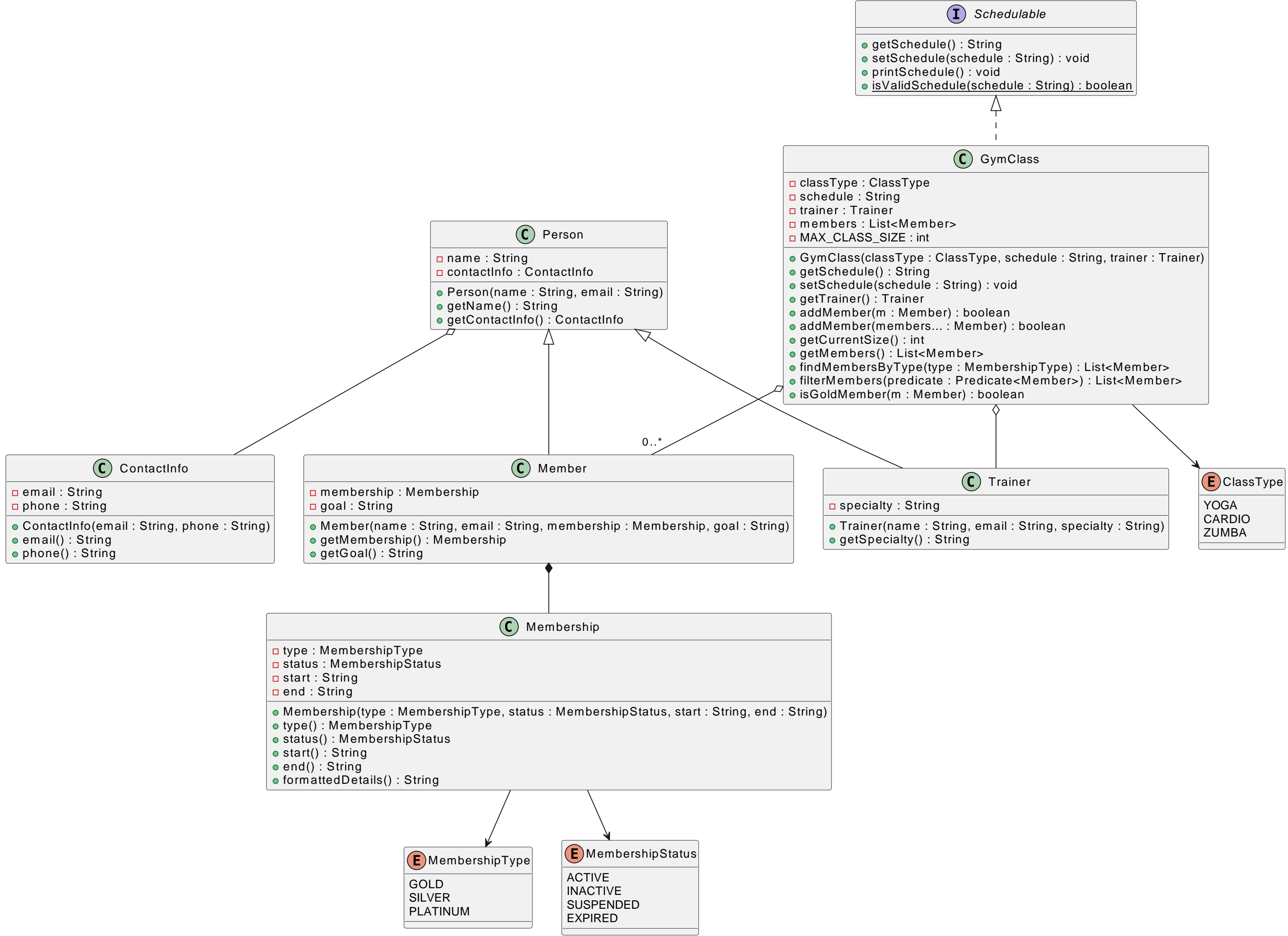
Gym Management System - Class Diagram
