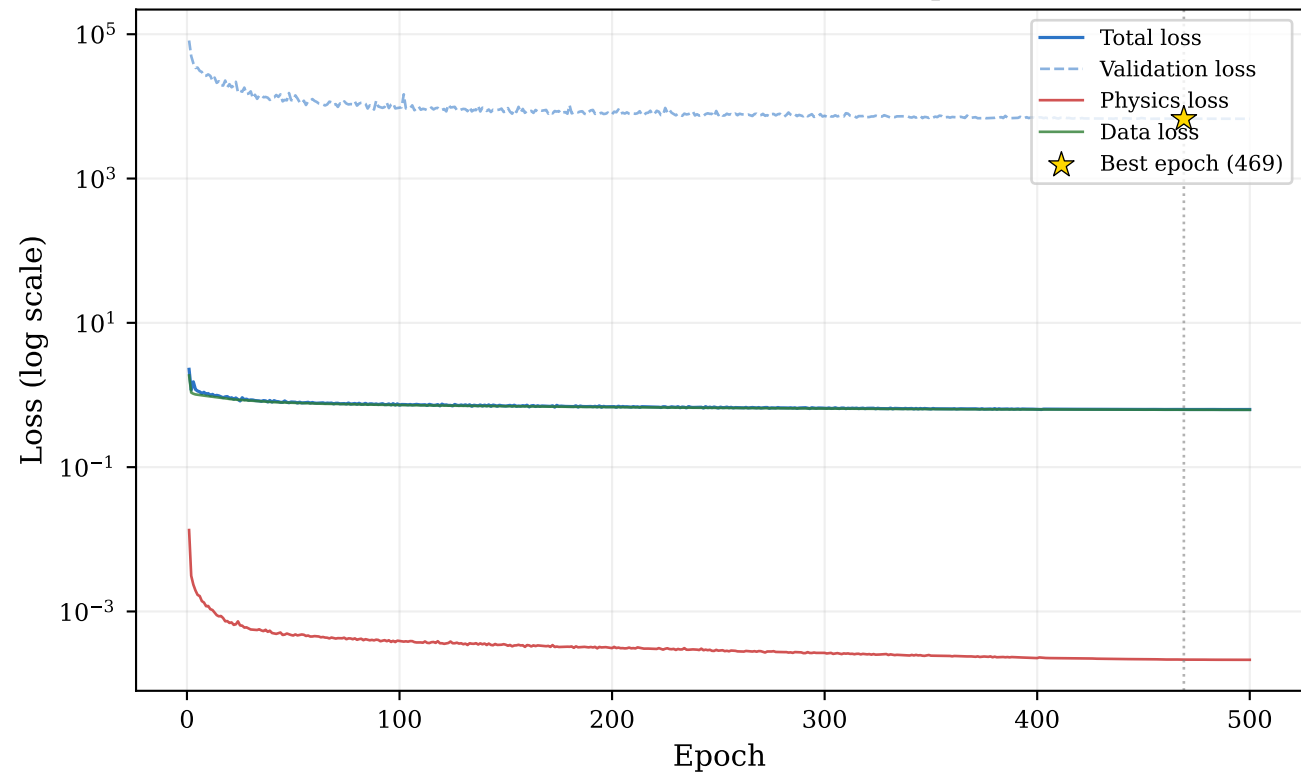
CCA Inverse PINN — Loss Decomposition
