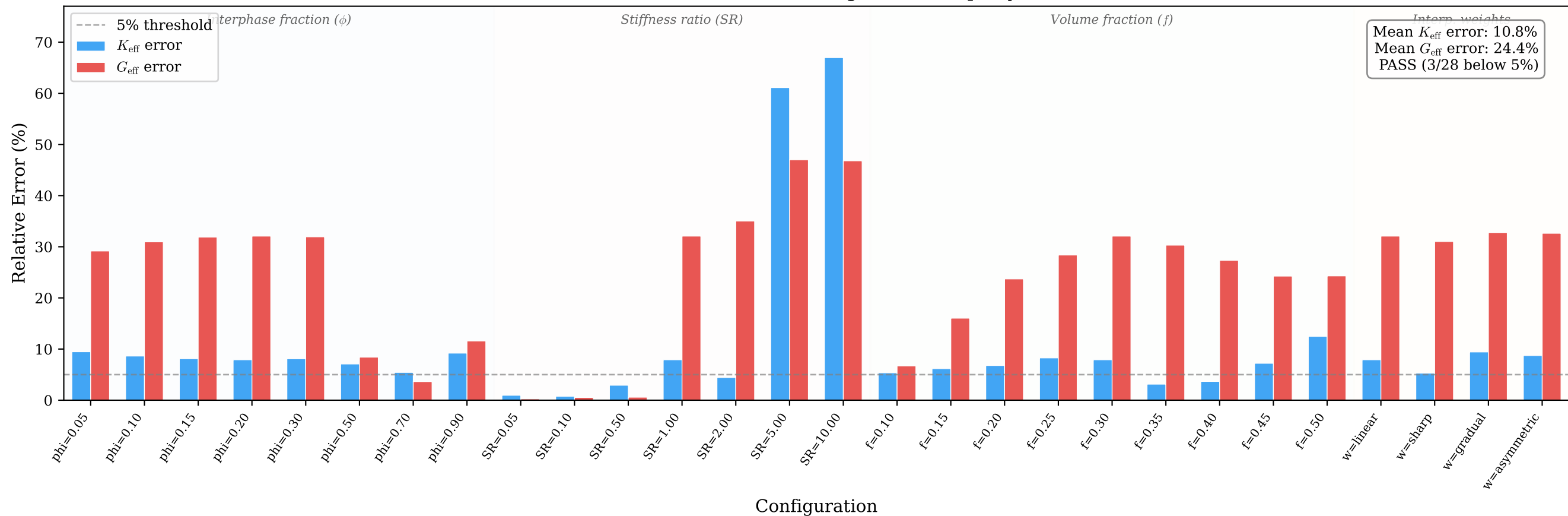
CSA Inverse PINN — Per-Configuration Property Errors
