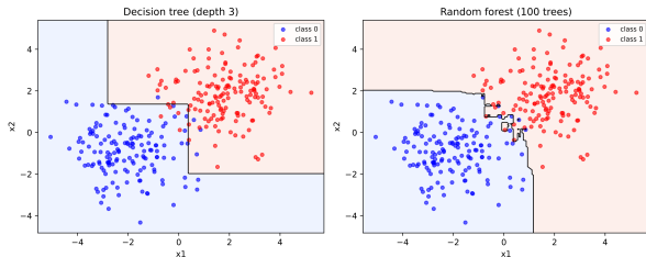
Decision boundary: one tree vs random forest
