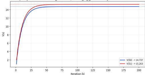
Iterative policy evaluation: starting from V=0 , converging geometrically to the closed-form solution
