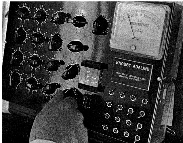
“Knobby ADALINE” — Stanford Electronics Labs, Stanford University (사진: Stanford Today, 1963)
