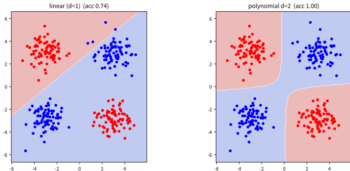
XOR quadrants: linear vs polynomial kernel degree 2
