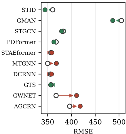
(a) volume: plain → injected RMSE capacity-law \rho=0.89 (log params, p=0.0005 )
