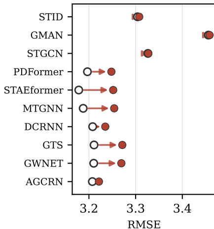
(b) speed: plain → injected RMSE capacity-law \rho=0.45 (log params, p=0.2 )
