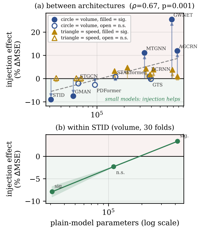
Fig. 6. Injection effect versus model capacity. (a) All ten architectures, both tasks, 30-fold: the effect rises with capacity from -9\% through zero near 10^5 parameters to +25\% , Spearman \rho = 0.67 ( p = 1.2 \times 10^{-3} ); filled markers are significant at p < 0.05 . (b) The same decay reproduced within STID by varying only hidden size (30 folds per point; the band spans the two seeds run at hidden 64), with architecture, training recipe and injected signal held fixed.
