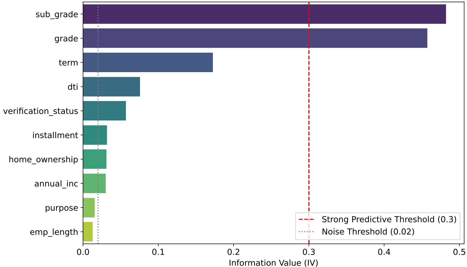
Information Value (IV) by Feature (Explainability Matrix)
