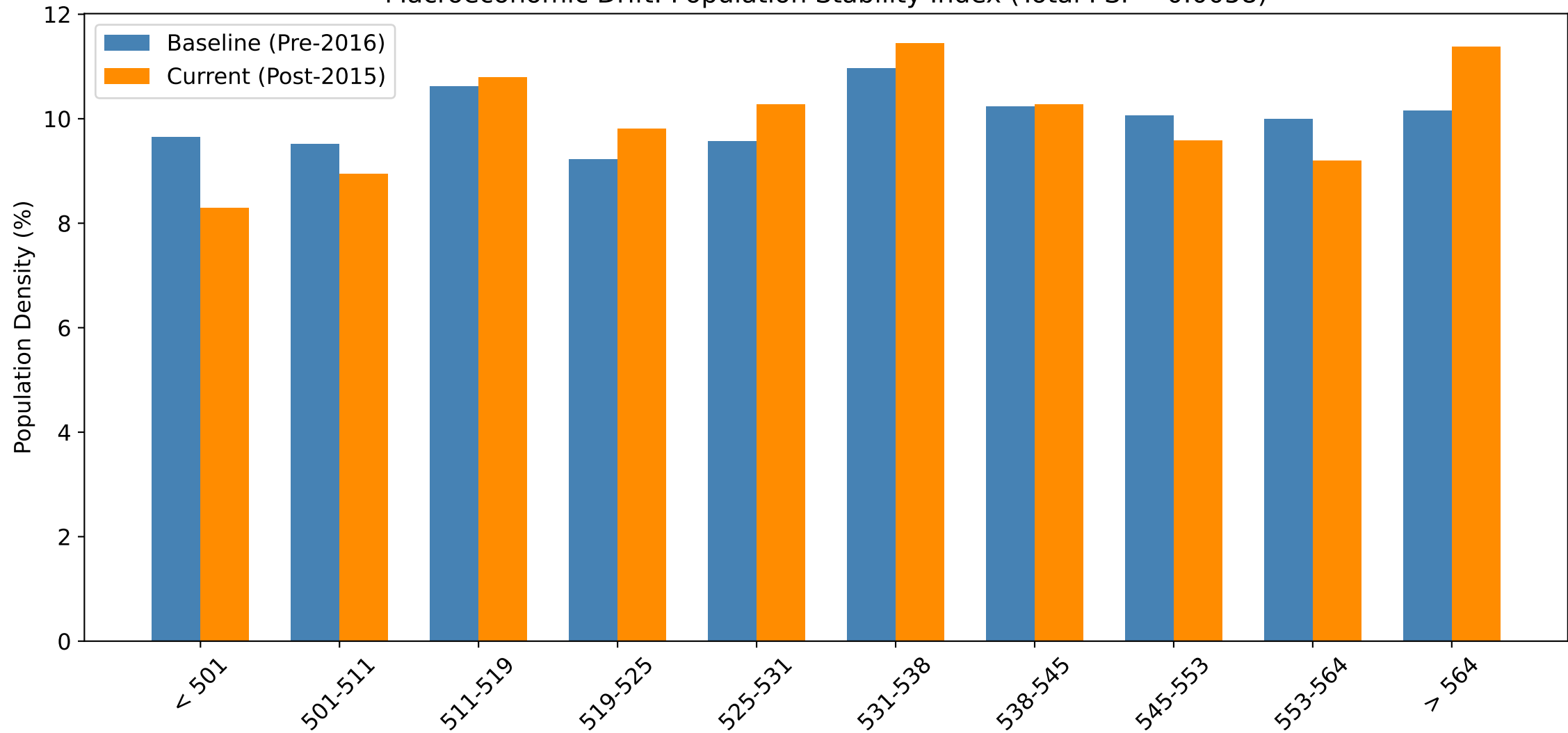
Macroeconomic Drift: Population Stability Index (Total PSI = 0.0058)
